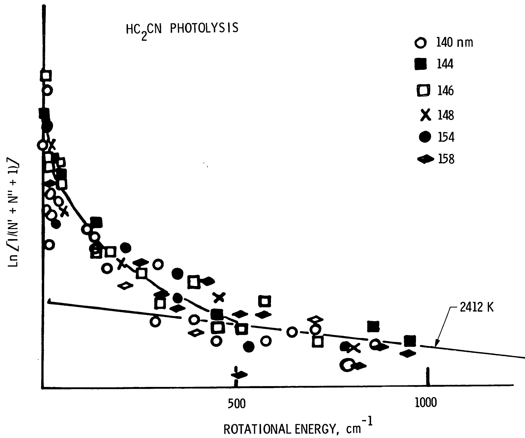
Figure 10. Boltzmann Plot of the rotational energy of the x state radical at the indicated wavelengths.
